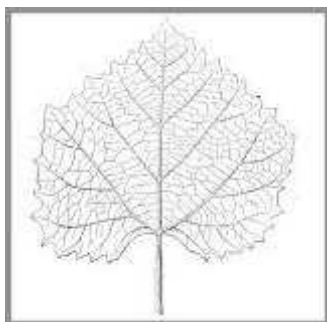
Vitis sezannensis , a vine leaf from the travertine of Sézanne (Fr) The viniculture is very proud of this fossil. It is the oldest vine leaf.
